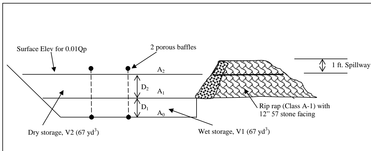
Figure 7.32-1 Sediment trap
