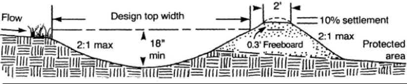
Diversion Berm Detail, Source: NCDENR Land Quality Section
