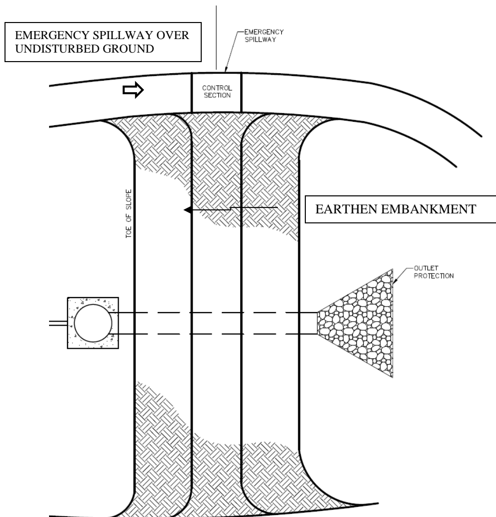
Figure 7.31-11 Earthen Embankment
